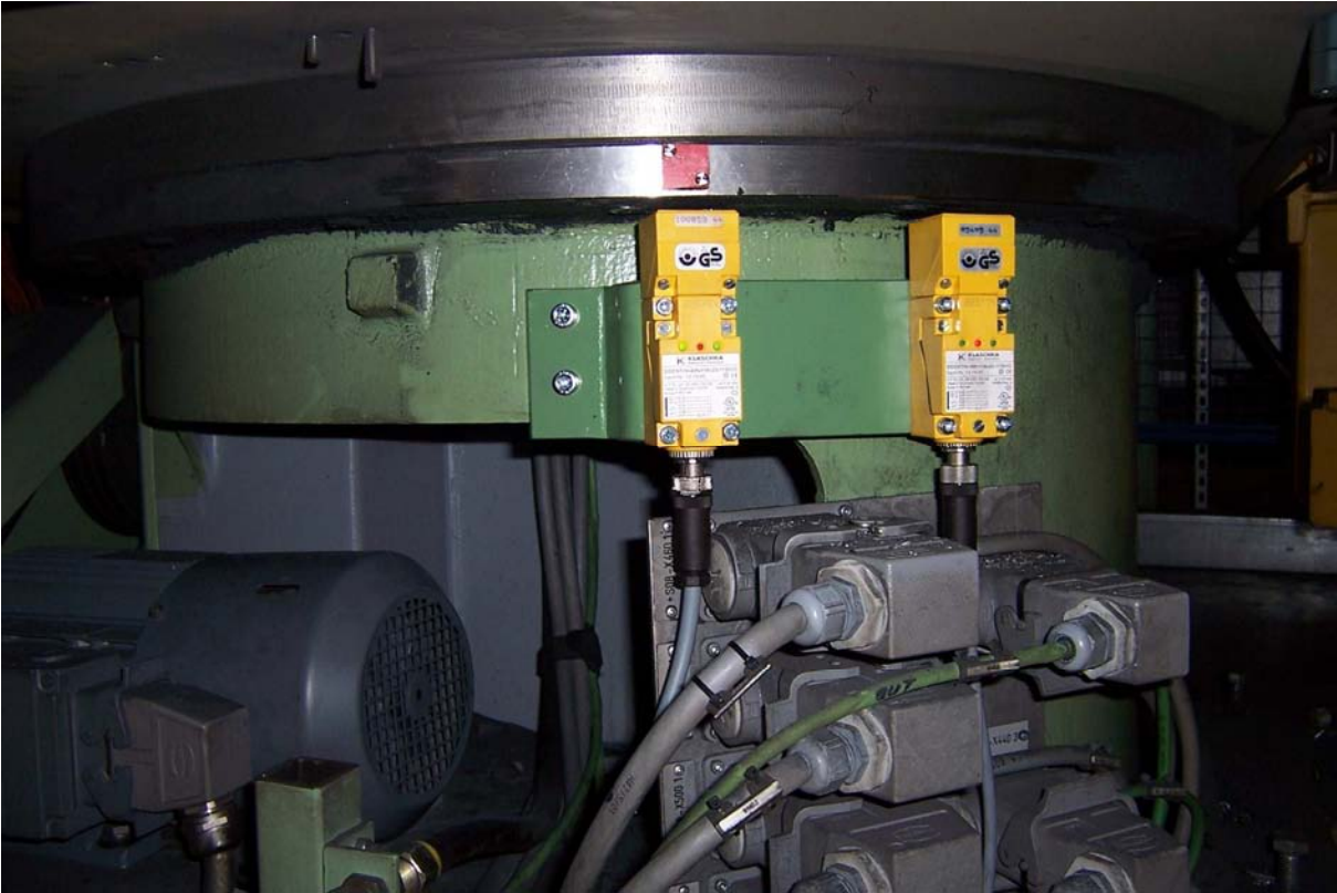
Tool positioning sensing system with safety function (control class IV)
